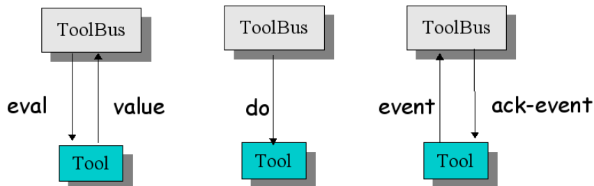
Figure 1.3. Communication between ToolBus and tools
